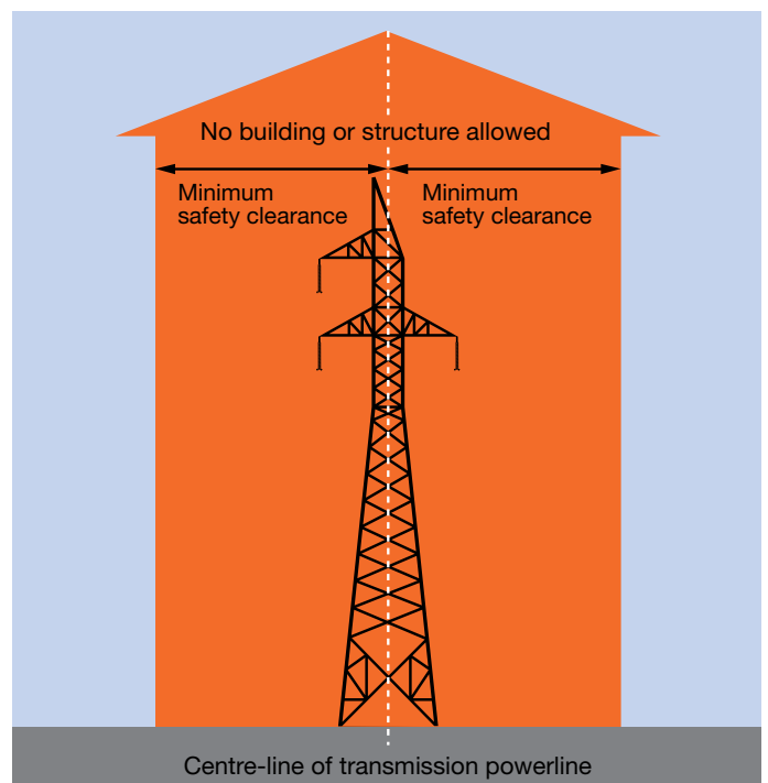
Image 3: Minimum safety clearance for transmission lines
